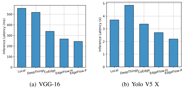
Fig. 6. Inference latency comparison with VGG-16 and Yolo V5 X.
