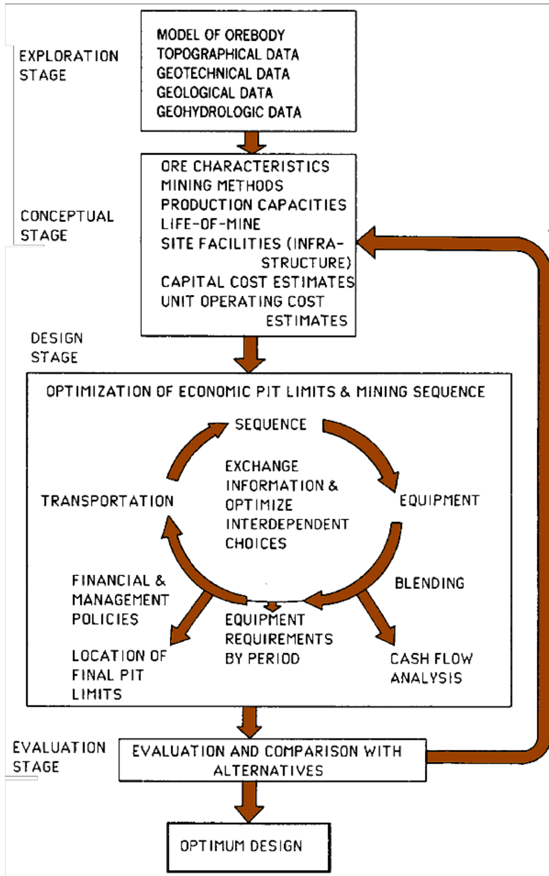
Fig: Diagrammatic presentation of the design process (after Fourie, 1992)
