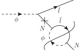
Fig. 7. Thermal cut in the \phi \rightarrow \bar{l}N decay, which gives rise to its purely-thermal L -violating CP-violation.
