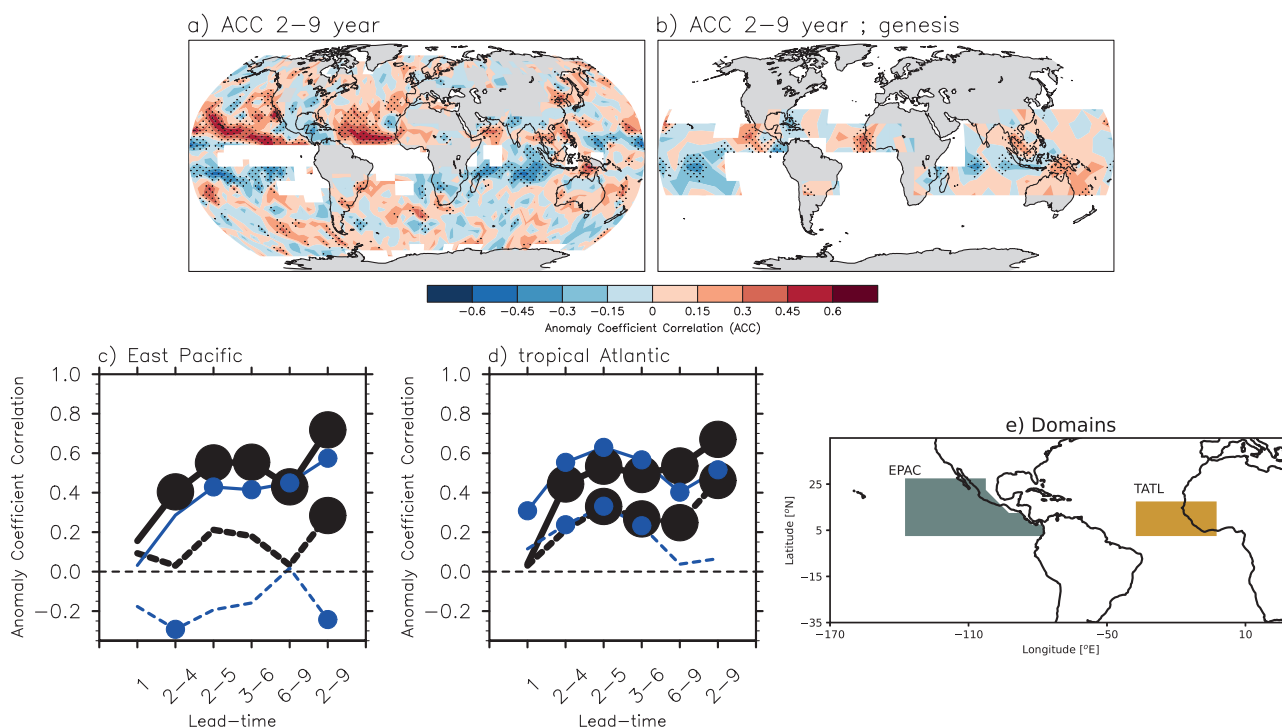
Fig. 2 | Skill in predicting TC activity. Skill (ACC) of DePreSys4 at the a 2–9 year forecast lead time (i.e., a decadal time window) for the track density. b as in a but for the TC genesis density. Stippling indicates that ACC is significantly different from zero according to a Monte–Carlo procedure with 5000 permutations and a 95% confidence level. Skill (ACC) in simulating the number of TC genesis in c the eastern Pacific and d tropical east Atlantic Ocean for the 1-year, 2–4, 2–5, 3–6, 6–9, and 2–9-year forecast lead times (i.e., in annual-to-decadal time windows). c, d The
